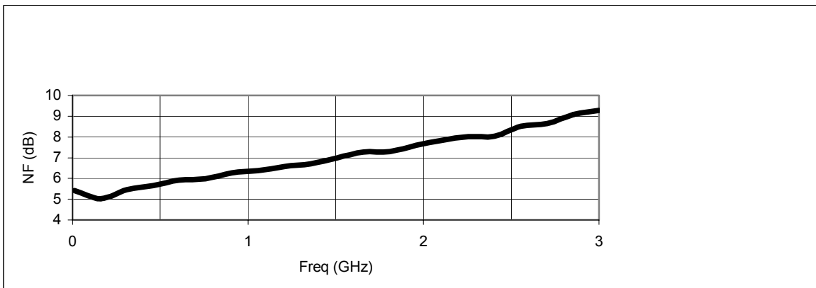
Nominal Instrument Noise Figure 10 MHz to 3 GHz Preamp On
