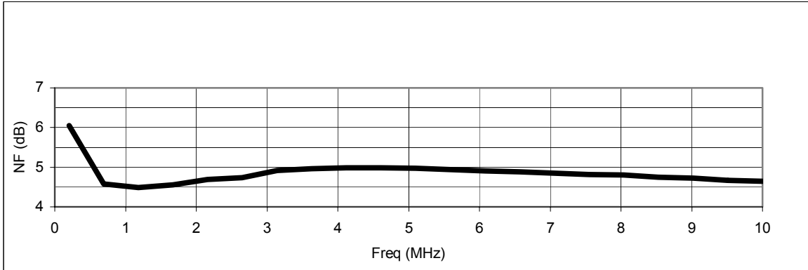
Nominal Instrument Noise Figure 200 kHz to 10 MHz Preamp On
